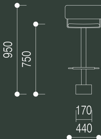
4 - with back stool with footrail
