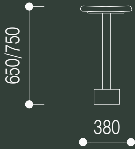
1 - no back stool, no footrail
