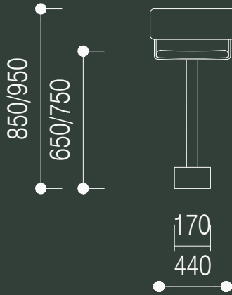
3 - with back stool, no footrail
