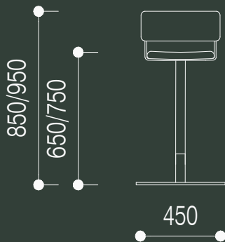
3 - with back stool, no footrail
