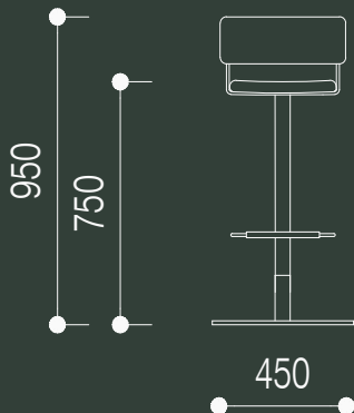
4 - with back stool with footrail
