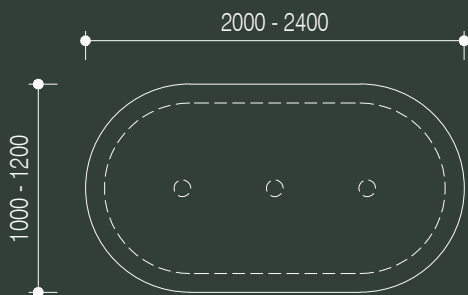
single row - pill shape
