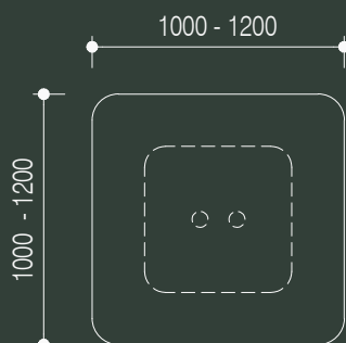
double row - square shape
