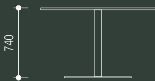
side elevation - double row
