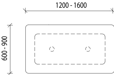
single row - rectangle shape
