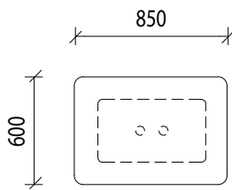
double row - rectangle shape
